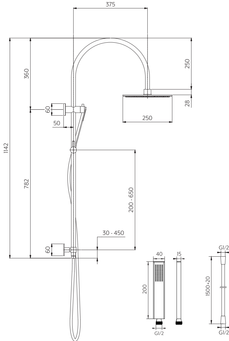
SIDE VIEW
