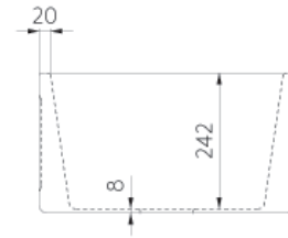
Side View (1:8)
