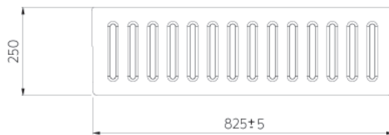
Front View (1:8)
