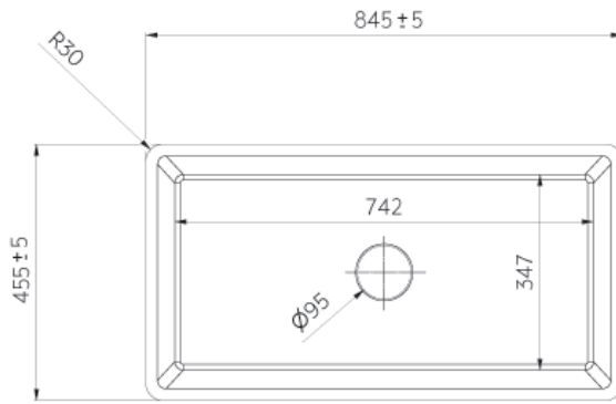
Top View (1:8)
