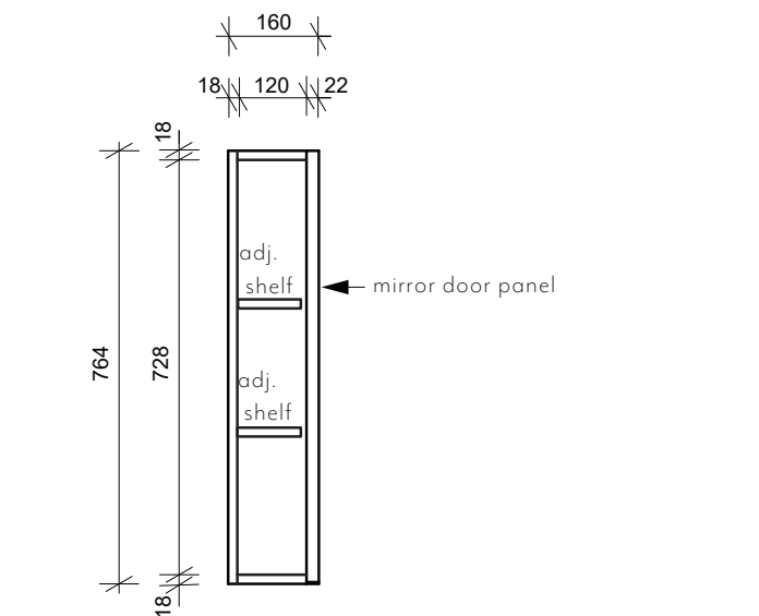
SIDE SECTION BB
