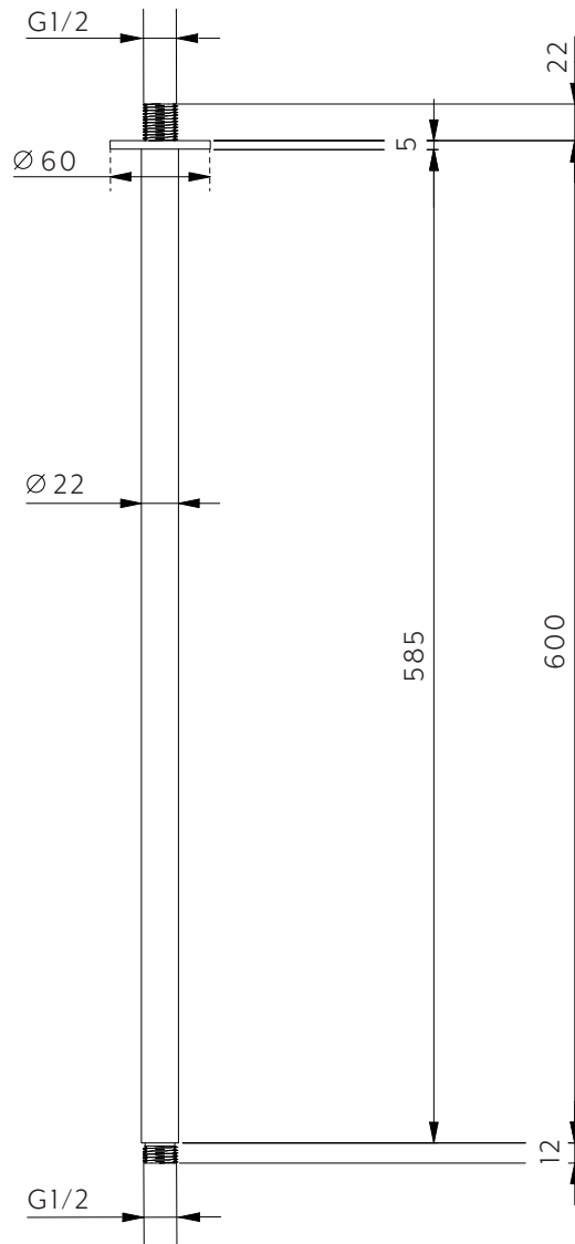
Front View
