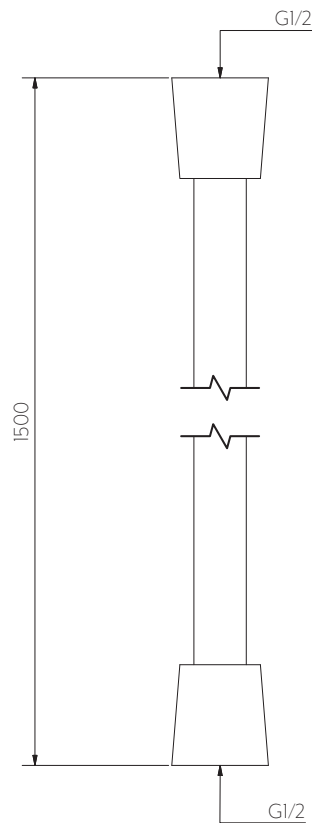
Front View (1:1)
